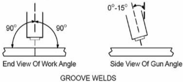
FIGURE 1: Proper Work and Gun Angles
